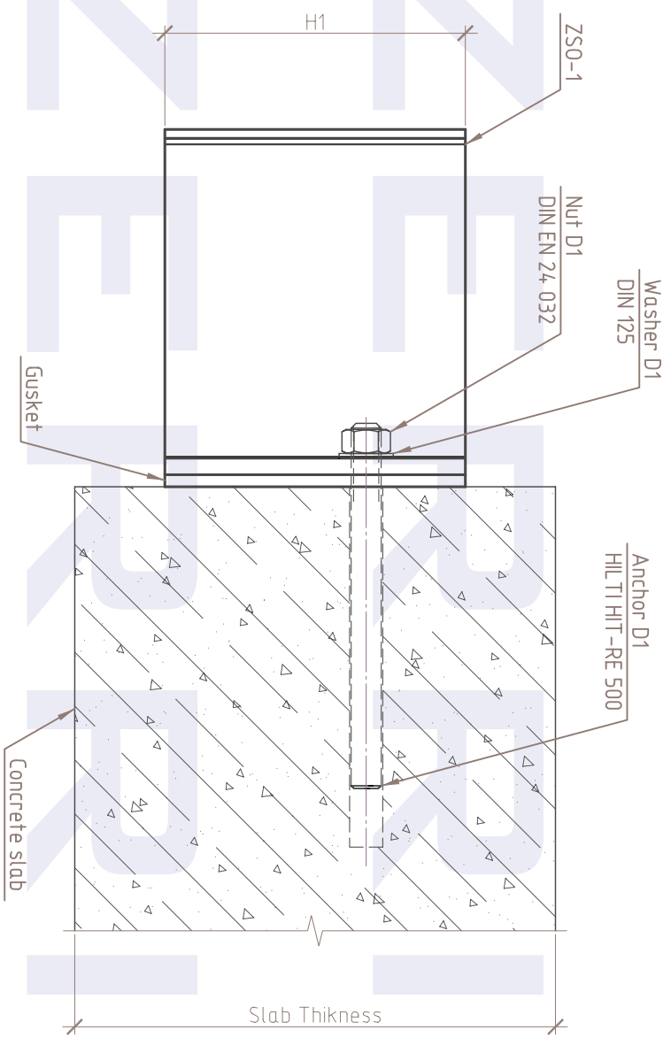
ELEVATION VIEW
